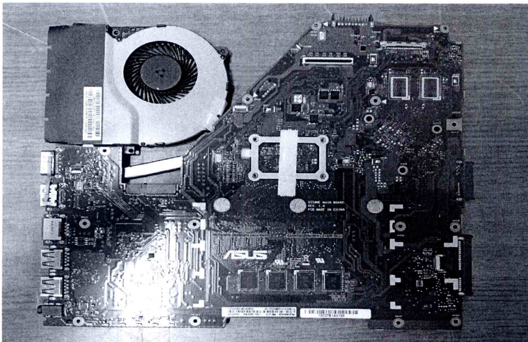
No.8 메인보드뒷면(X550WE_Conf_H)
