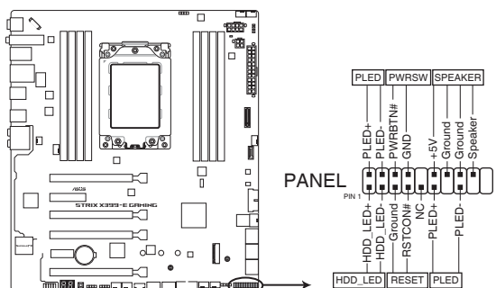
ROG STRIX X399-E GAMING System panel connector
