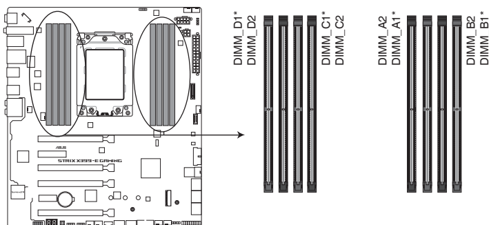
ROG STRIX X399-E GAMING 288-pin DDR4 DIMM sockets
