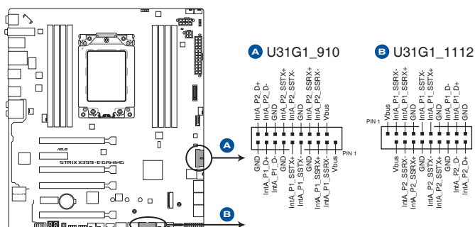
ROG STRIX X399-E GAMING USB 3.1 Gen 1 connectors
