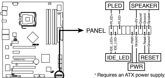
P5N32-E SLI System panel connector
