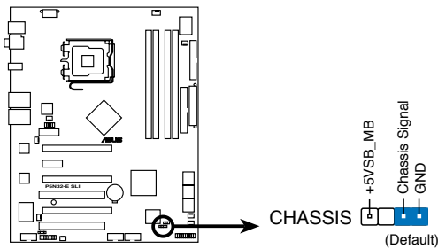
P5N32-E SLI Chassis intrusion connector
