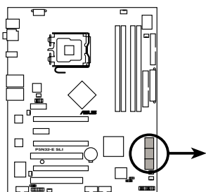
P5N32-E SLI SATA connectors
