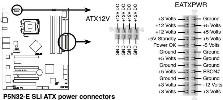
P5N32-E SLI ATX power connectors
