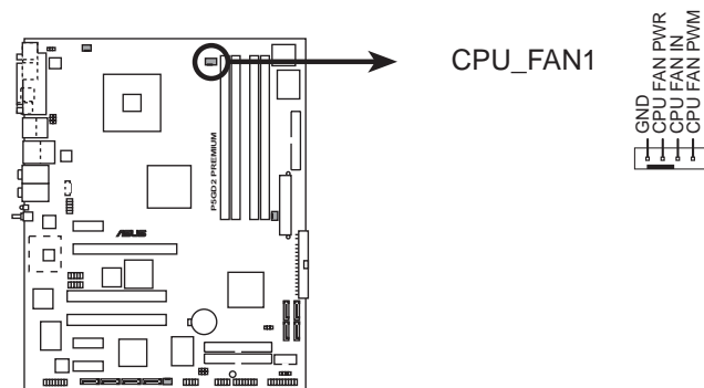
P5GD2 PREMIUM CPU Fan connector
