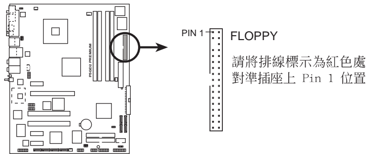
P5GD2 PREMIUM Floppy disk drive connector
