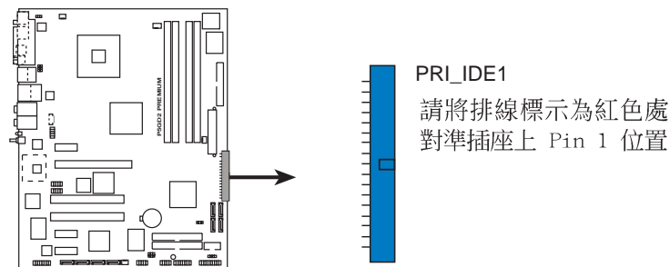
P5GD2 PREMIUM IDE connector
