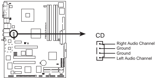
P5GD2 Premium CD audio connector
