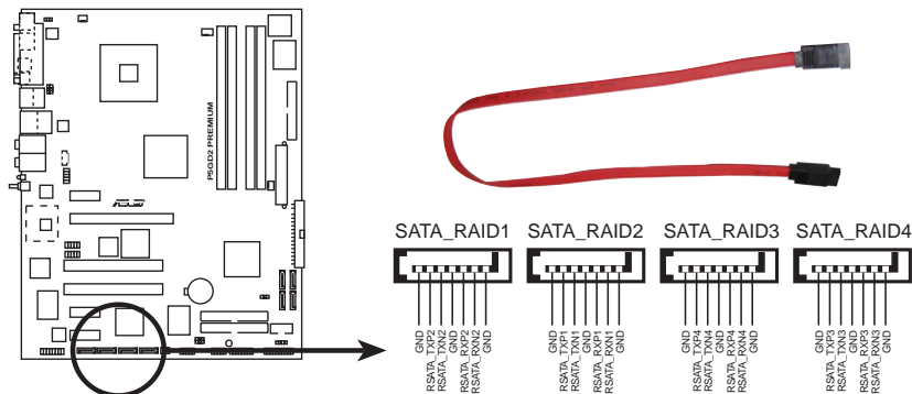
P5GD2 PREMIUM SATA RAID connectors
