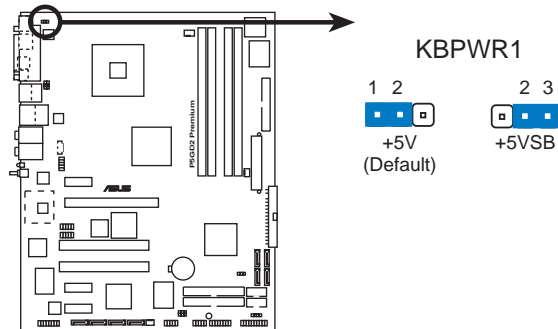
P5GD2 Premium Keyboard power setting
