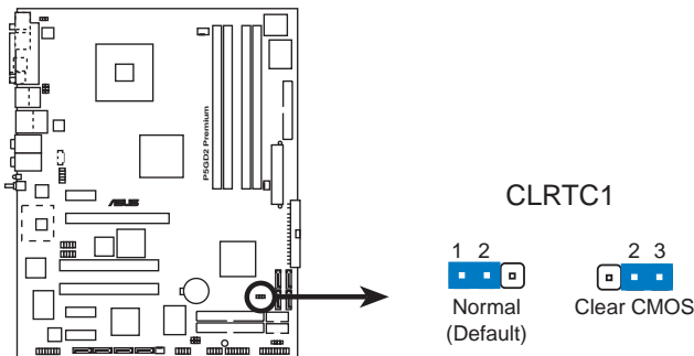
P5GD2 Premium Clear RTC RAM
