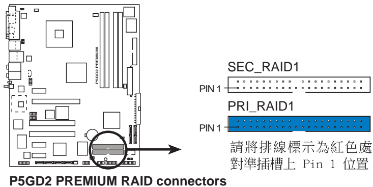
P5GD2 PREMIUM RAID connectors
