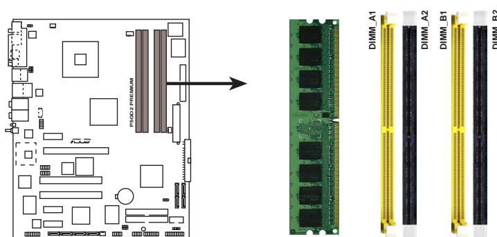
P5GD2 PREMIUM 184-Pin DDR DIMM sockets
