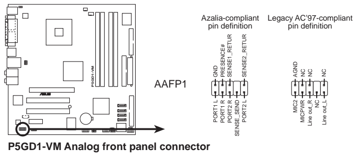
P5GD1-VM Analog front panel connector
