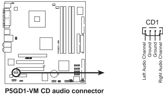
P5GD1-VM CD audio connector
