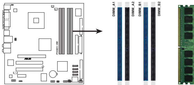
P5GD1-VM 184-Pin DDR DIMM Sockets
