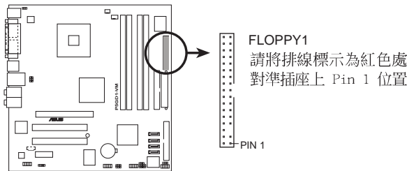
P5GD1-VM Floppy disk drive connector
