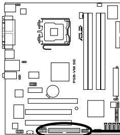
P5B-VM SE EIDE Connector
