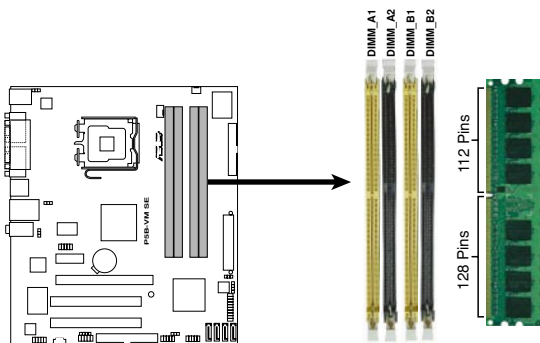
P5B-VM SE 240-pin DDR2 DIMM Sockets
