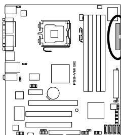
P5B-VM SE Floppy Disk Drive Connector
