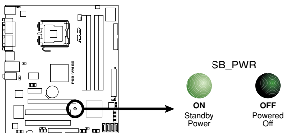
P5B-VM SE Onboard LED
