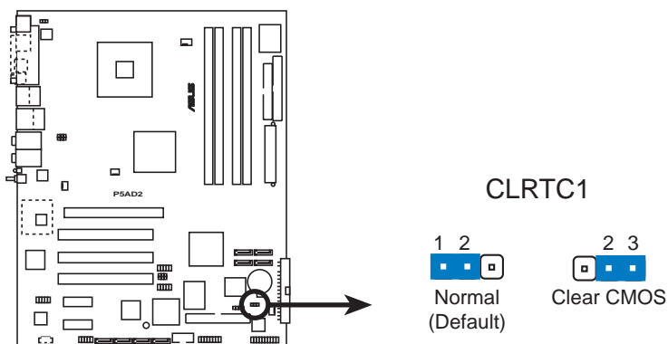
P5AD2 Deluxe Clear RTC RAM
