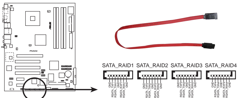
P5AD2 Deluxe SATA RAID connectors
