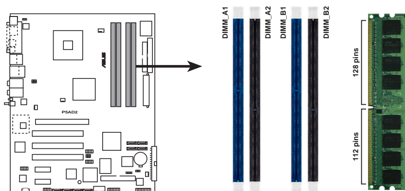
P5AD2 Deluxe DDR2 DIMM sockets
