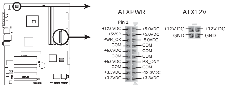
K8V-X ATX Power Connectors
