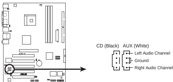
K8V-X Internal Audio Connectors
