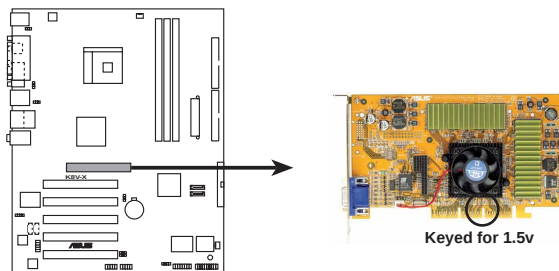
K8V-X Accelerated Graphics Port (AGP)
