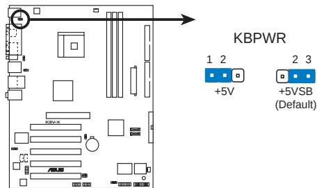
K8V-X Keyboard Power Setting
