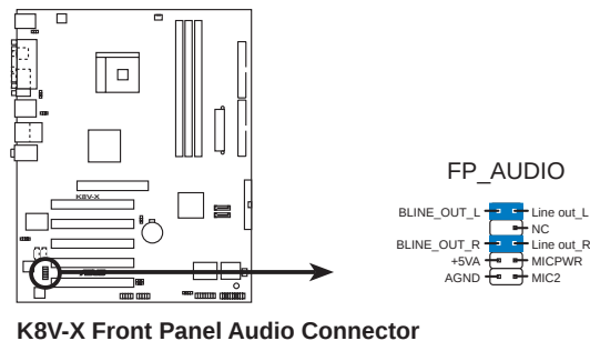
K8V-X Front Panel Audio Connector
