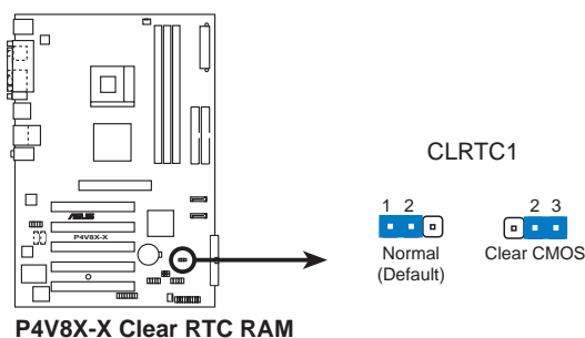
P4V8X-X Clear RTC RAM
