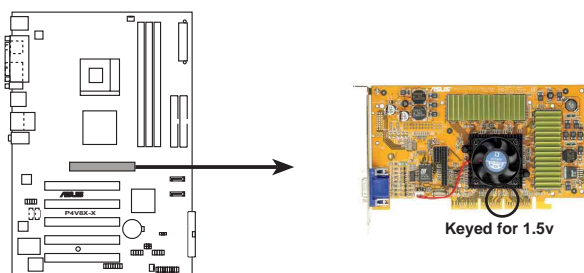
P4V8X-X Accelerated Graphics Port (AGP)
