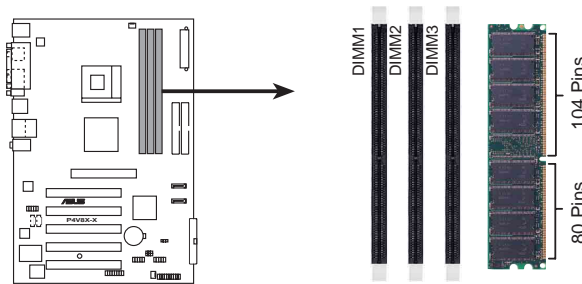
P4V8X-X 184-Pin DDR DIMM Sockets
