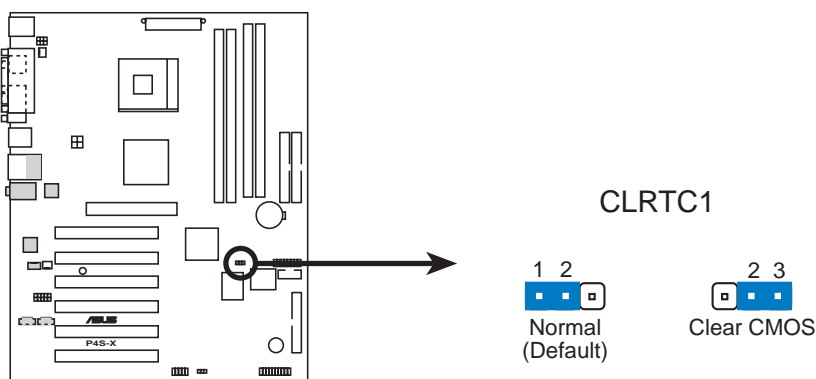
P4S-X Clear RTC RAM Setting
