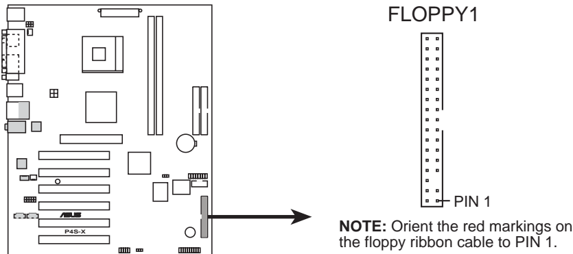
P4S-X Floppy Disk Drive Connector
