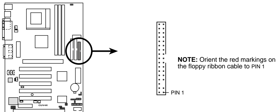
CUV4X Floppy Disk Drive Connector
