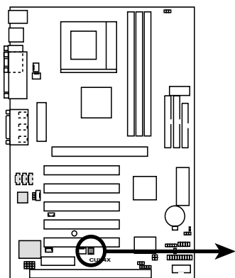
CUV4X Wake-On-Ring Connector
