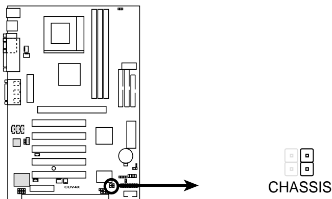
CUV4X Chassis Open Alarm Lead
