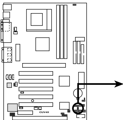
CUV4X IDE Activity LED
