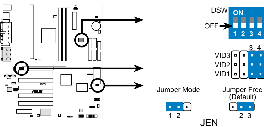
K7V Jumper Mode Setting
