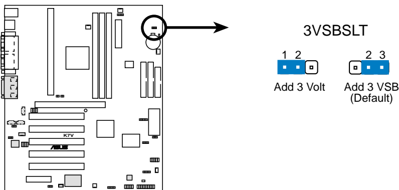
K7V PCI 3Volt Selection
