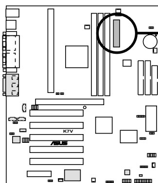
K7V ATX Power Connector
