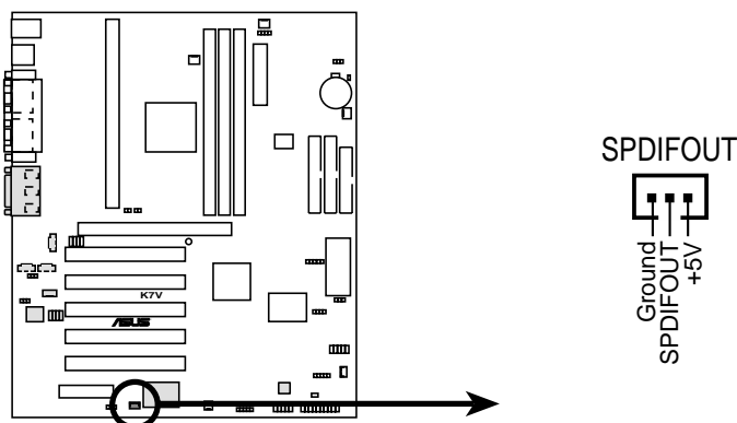
K7V Audio Digital Interface Connector
