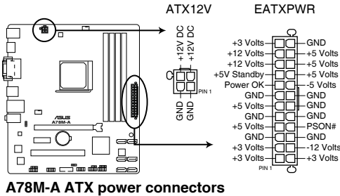
A78M-A ATX power connectors
