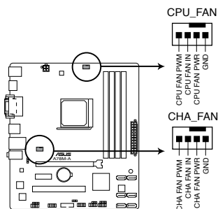
A78M-A Fan connectors
