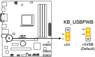
A78M-A Keyboard and USB device wake up
