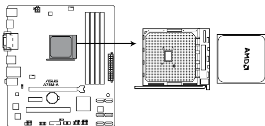
A78M-A CPU socket FM2+
