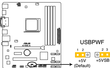
A78M-A USB device wake up
