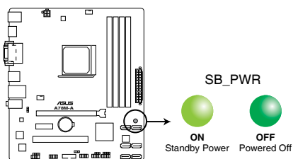
A78M-A Onboard LED
