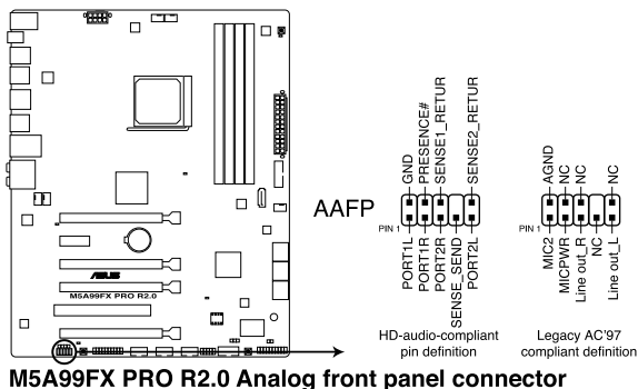
M5A99FX PRO R2.0 Analog front panel connector
