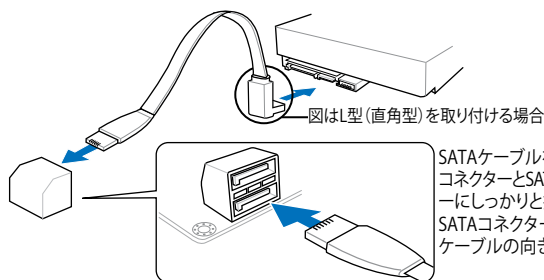
M5A99FX PRO R2.0 SATA 6.0 Gb/s connectors
