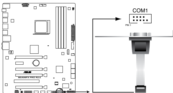
M5A99FX PRO R2.0 Serial port (COM1) connector
