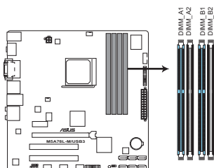
M5A78L-M/USB3 240-pin DDR3 DIMM sockets
