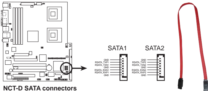
NCT-D SATA connectors
