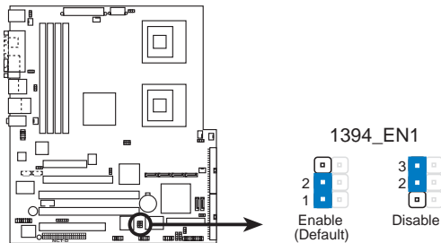
NCT-D 1394 Function setting
