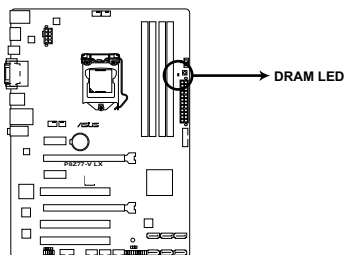
LED DRAM de la P8Z77-V LX
