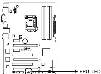
LED EPU de la P8Z77-V LK
