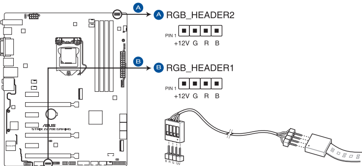
STRIX Z270E GAMING RGB_HEADER connectors
