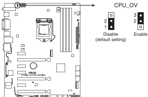
STRIX Z270E GAMING CPU_OV setting
