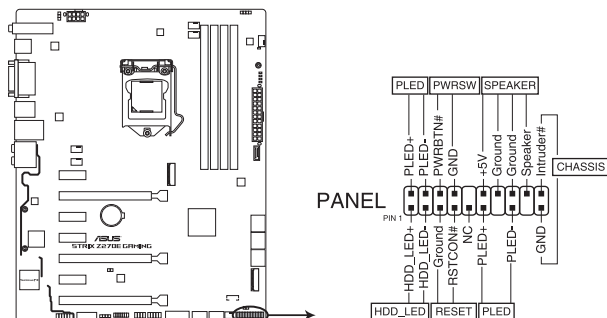
STRIX Z270E GAMING System panel connector
