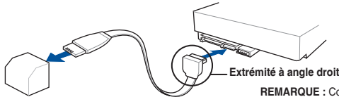
STRIX Z270E GAMING Intel® SATA 6 Gb/s connectors
