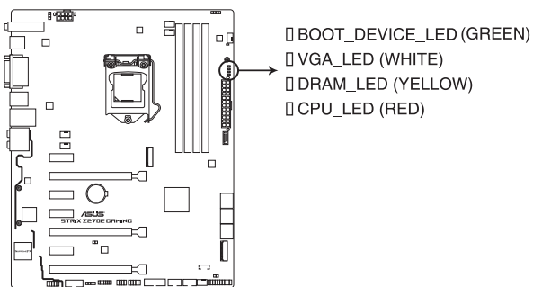
STRIX Z270E GAMING CPU/ DRAM/ BOOT_DEVICE/ VGA LED
