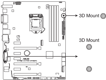
STRIX Z270E GAMING 3D Printing Mount
