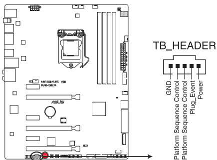
MAXIMUS VIII RANGER TB_HEADER connector
