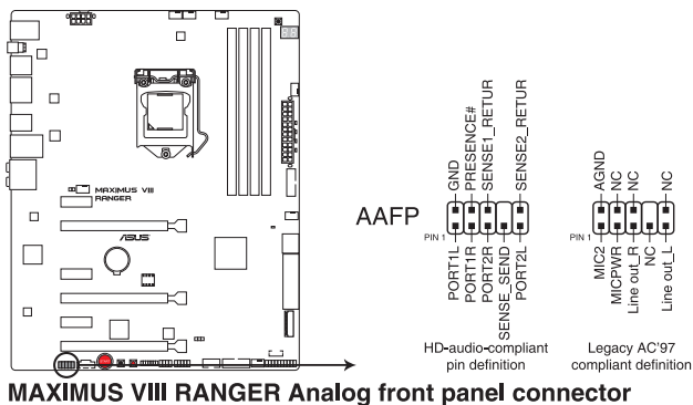
MAXIMUS VIII RANGER Analog front panel connector
