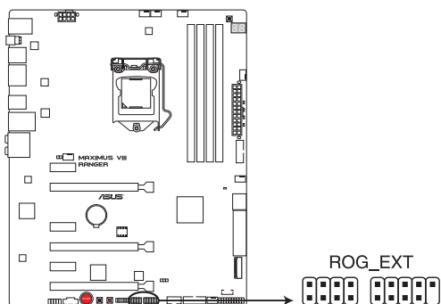
MAXIMUS VIII RANGER ROG_EXT connectors
