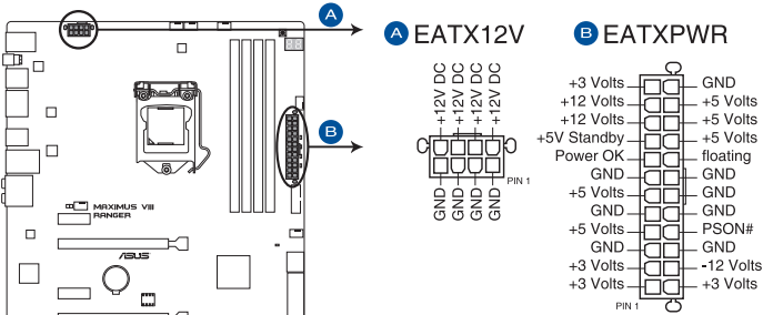
MAXIMUS VIII RANGER ATX power connectors
