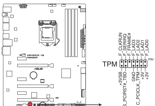
MAXIMUS VIII RANGER TPM connector
