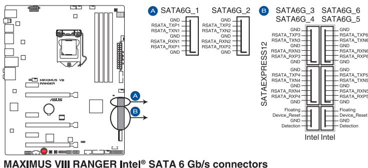
MAXIMUS VIII RANGER Intel® SATA 6 Gb/s connectors
