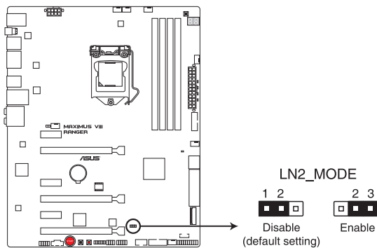
MAXIMUS VIII RANGER LN2_MODE setting
