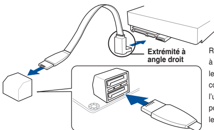
MAXIMUS VIII RANGER Intel® SATA 6 Gb/s connectors
