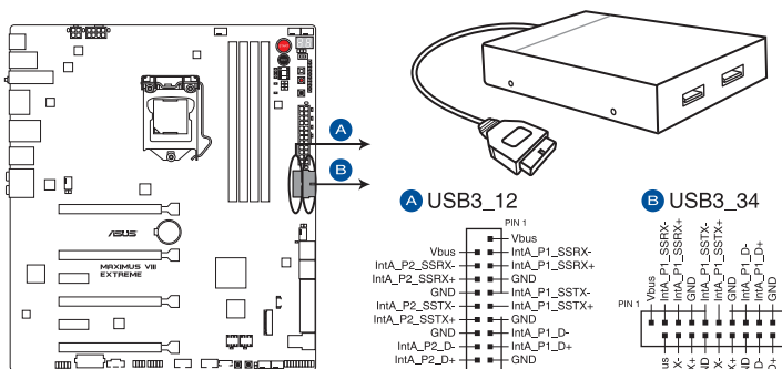
MAXIMUS VIII EXTREME USB3.0 connectors
