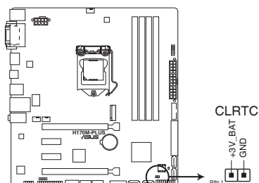
H170M-PLUS Clear RTC RAM
