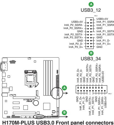
H170M-PLUS USB3.0 Front panel connectors
