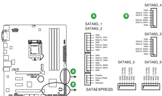
H170M-PLUS Intel® SATA 6.0Gb/s connectors
