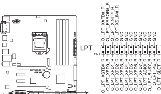
H170M-PLUS Parallel Port connector
