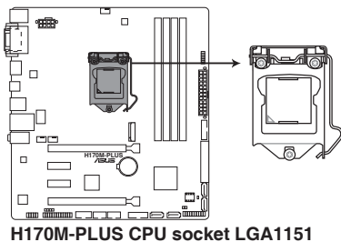
H170M-PLUS CPU socket LGA1151
