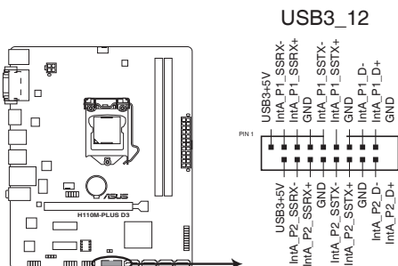
H110M-PLUS D3 USB3.0 Front panel connector
