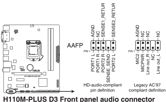
H110M-PLUS D3 Front panel audio connector
