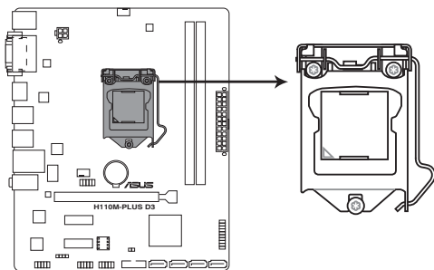
H110M-PLUS D3 CPU socket LGA1151
