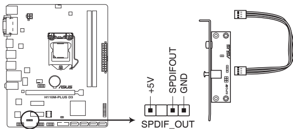
H110M-PLUS D3 Digital audio connector
