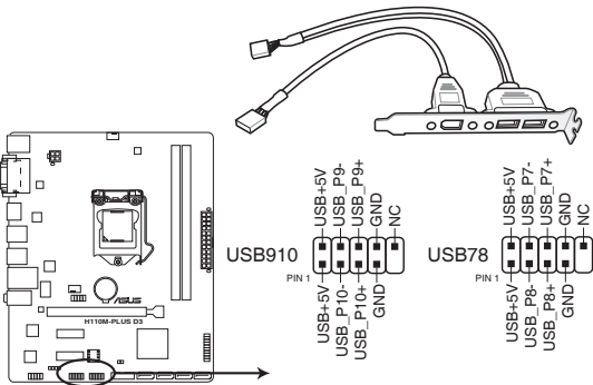
H110M-PLUS D3 USB2.0 connectors
