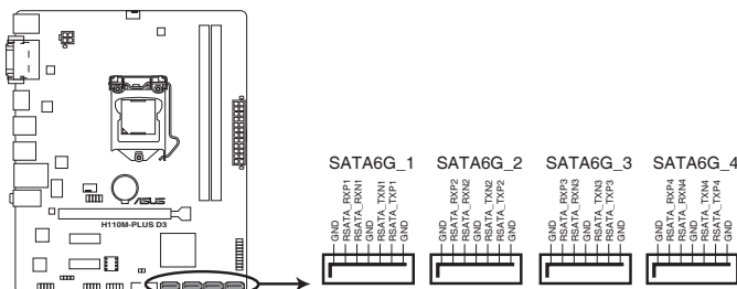
H110M-PLUS D3 SATA 6.0Gb/s connectors
