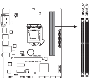
H110M-PLUS D3 240-pin DDR3 DIMM sockets
