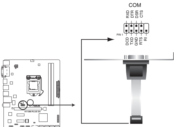
H110M-PLUS D3 Serial port (COM) connector
