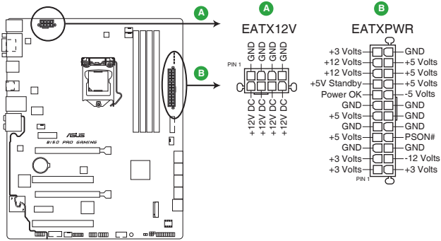
B150 PRO GAMING ATX power connectors
