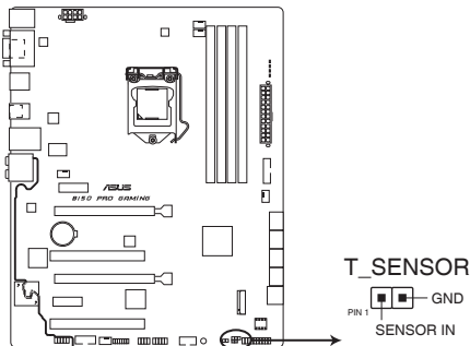
B150 PRO GAMING T_SENSOR connector
