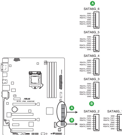
B150 PRO GAMING Intel® SATA 6.0Gb/s connectors
