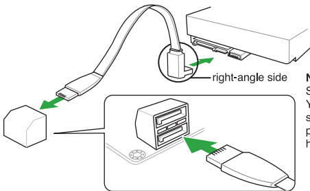
B150 PRO GAMING Intel® SATA 6.0Gb/s connectors
