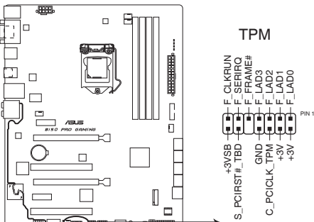
B150 PRO GAMING TPM connector
