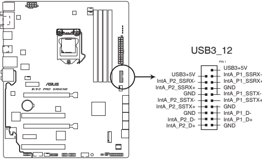
B150 PRO GAMING USB3.0 Front panel connector
