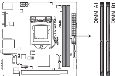
B150I PRO GAMING/AURA 288-pin DDR4 DIMM socket
