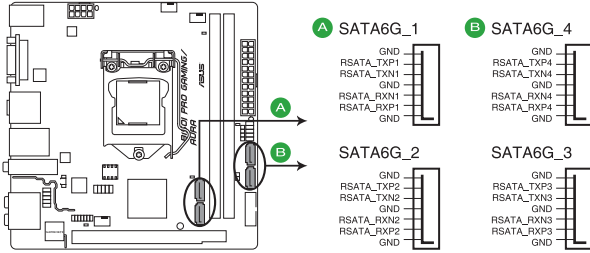
B150I PRO GAMING/AURA Intel® SATA 6 Gb/s connectors
