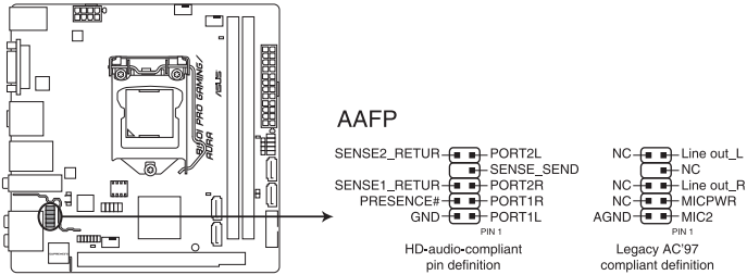
B150I PRO GAMING/AURA Analog front panel connector
