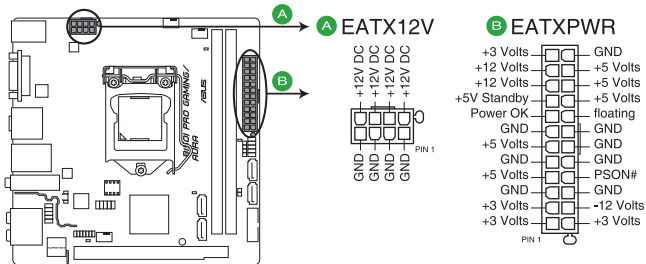
B150I PRO GAMING/AURA ATX power connectors
