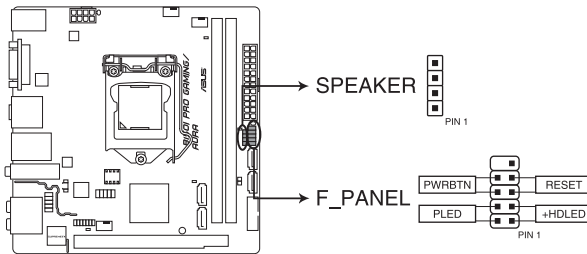
B150I PRO GAMING/AURA SPEAKER & F_PANEL connectors
