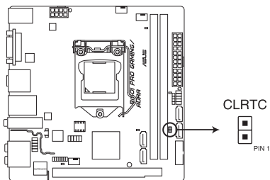
B150I PRO GAMING/AURA CLRTC
