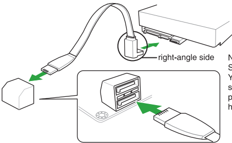
B150I PRO GAMING/AURA Intel® SATA 6 Gb/s connectors
