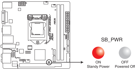
B150I PRO GAMING/AURA Onboard LED
