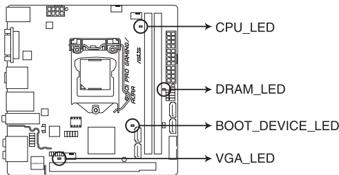
B150I PRO GAMING/AURA CPU/ DRAM/ BOOT_DEVICE/ VGA LED
