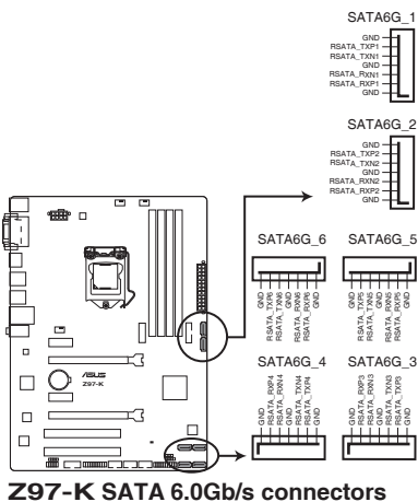
Z97-K SATA 6.0Gb/s connectors
