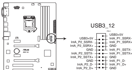
Z97-K USB3.0 front panel connector
