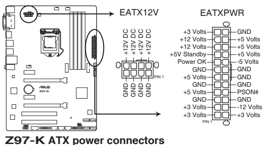
Z97-K ATX power connectors
