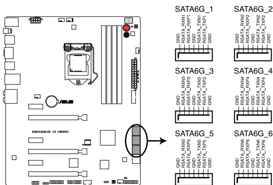
MAXIMUS VI HERO Intel® SATA 6Gb/s connectors
