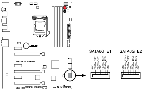
MAXIMUS VI HERO Asmedia® SATA 6 Gb/s connectors
