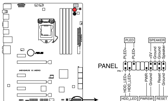
MAXIMUS VI HERO System panel connector
