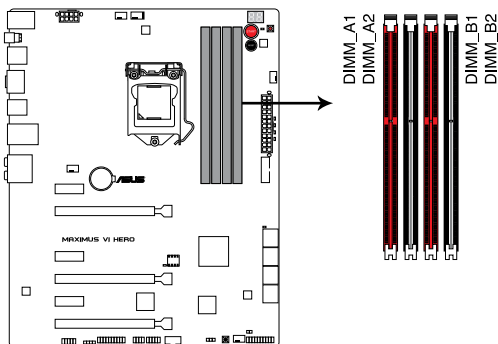
MAXIMUS VI HERO 240-pin DDR3 DIMM slots
