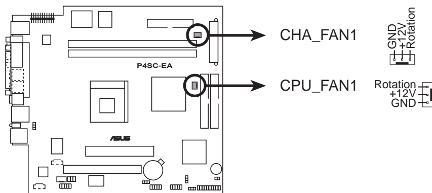
P4SC-EA 12-Volt Cooling Fan Power
